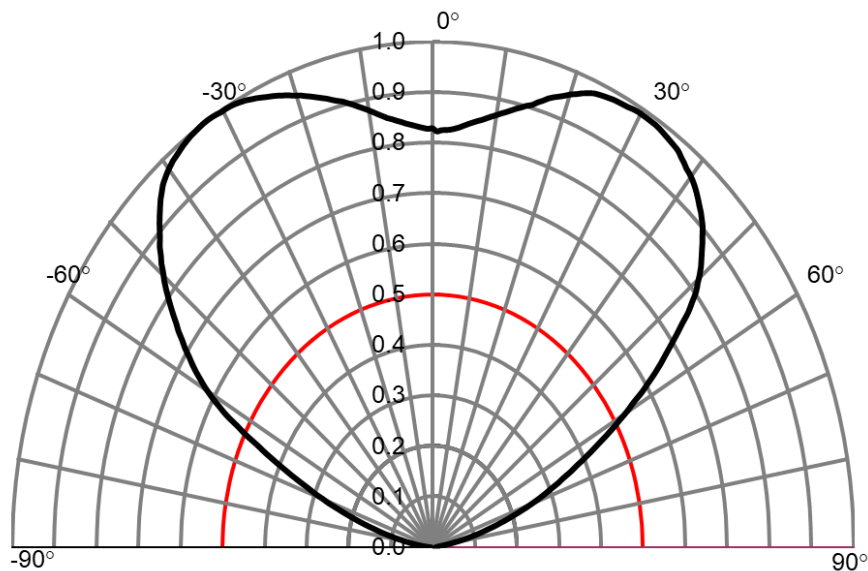
Fig 5. Radiation Characteristics
